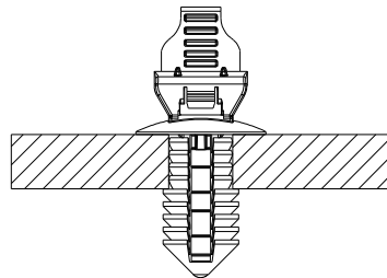
ASSEMBLED VIEW
